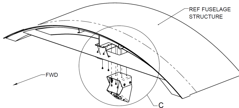
Figure 11: Camera Mounting
