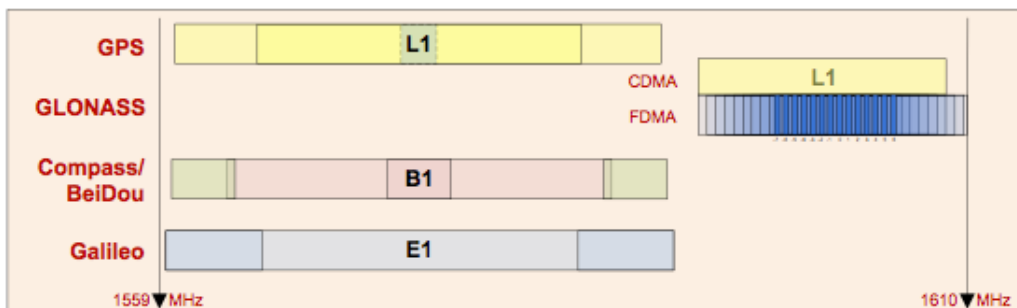
Figure D-2: Frequencies used by Core Constellations
