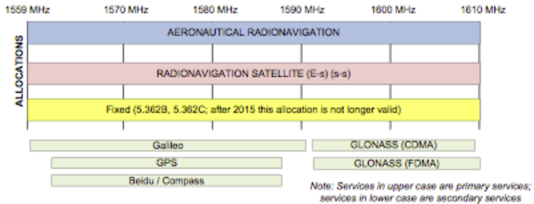
Figure D-2: Frequencies used by Core Constellations
